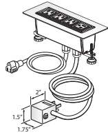
EUB1-SLOB-4000 4-Port IEC-Cord and Power Cord Breaker Plug
