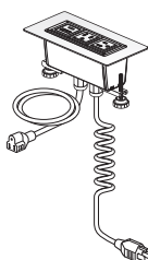
EUB1-SF0B-2100 3-Port IEC-Cord and Spiral Cord
