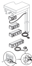
EUS1-PF0B EUS1-PF0W EUS1-HLOB EUS1-HLOW Seamless Enhanced Power Module
