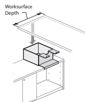
Desk to Storage Bracket
